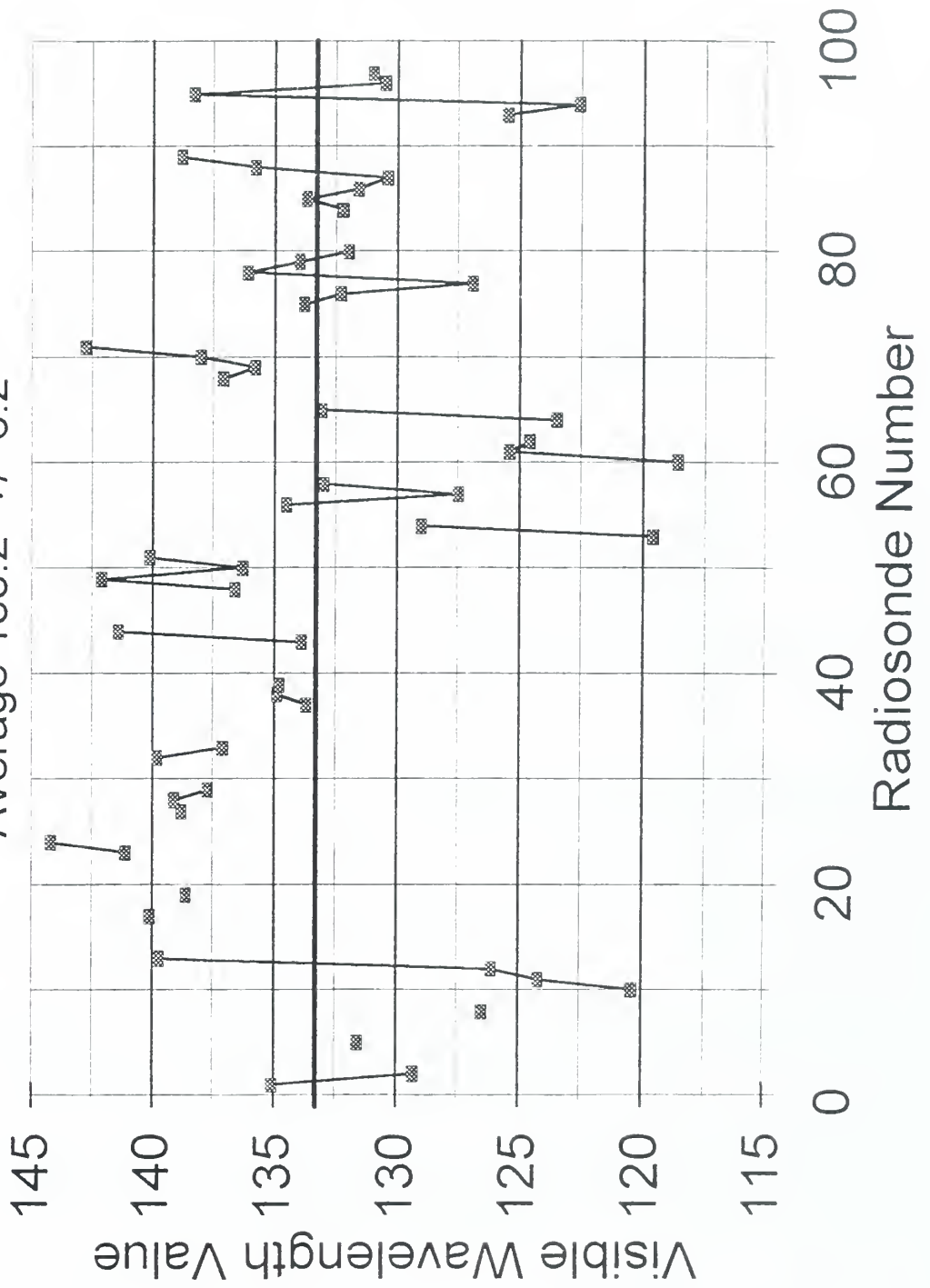
Figure 5.13 Visible Wavelength Water Vapor Calibration Values
