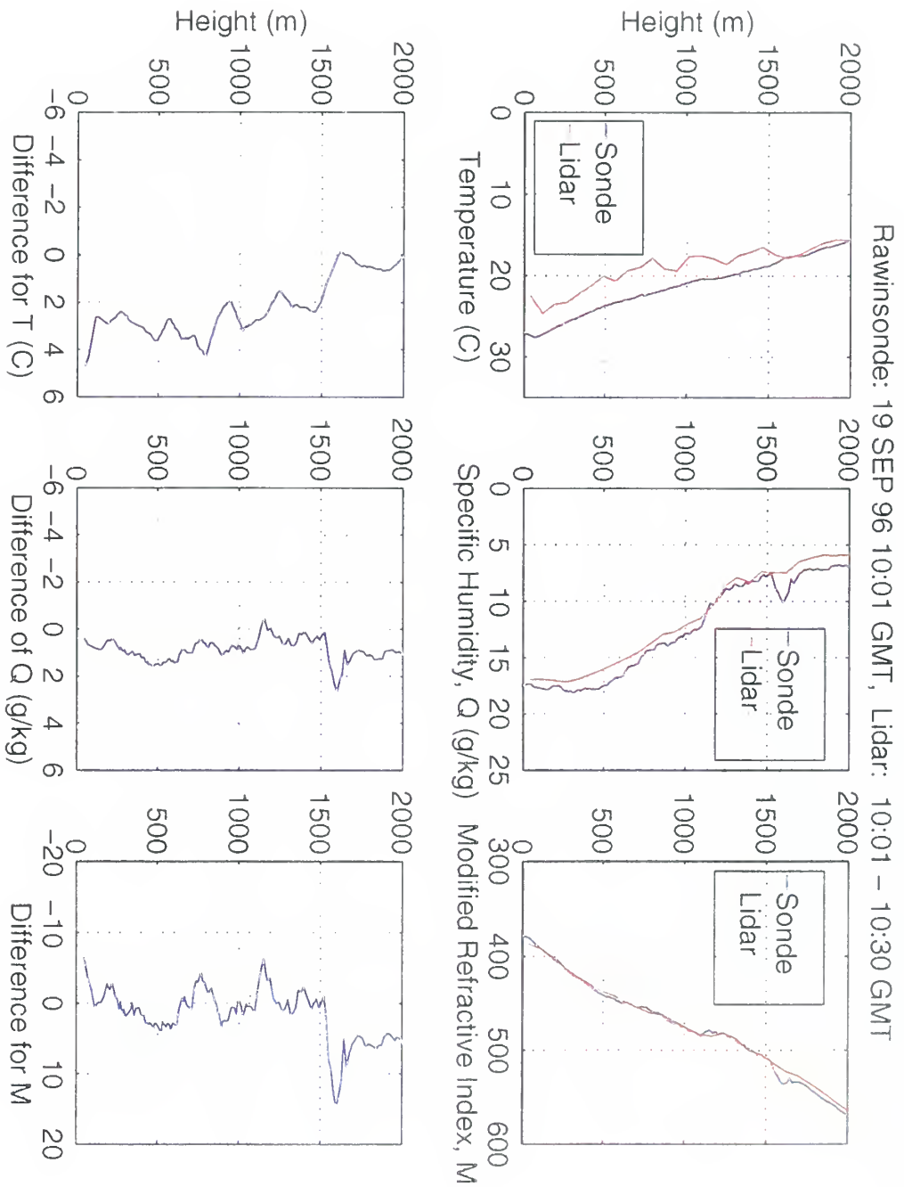
Figure 5.10 Same as Figure 5.3 for 19 Sep 96 data
