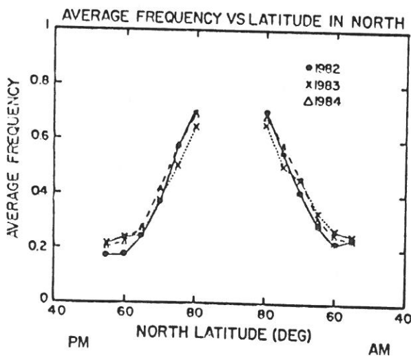
Fig. 6. Average occurrence frequency of PMC determined by the SME UV spectrometer for 3 northern summer seasons. The data have been merged in the interval, 44 days before solstice to 60 days after solstice.
