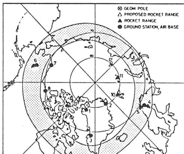
Fig. 8. Proposed stations for Super CAMP for rocket launches (triangle), ground based experiments and airplanes (circles). The different allocations are Thule, Greenland (1), Nord, Greenland (2), Søndre Strømfjord, Greenland (3), Kiruna (Esrang, Eiscat), Sweden (4), Andenes, Norway (5), Poker Flat, Alaska (6), Pt. Barrow, Alaska (7), Cape Perry, Canada (8), Resolute Bay, Canada (9), Spitzbergen (10), Heiss Island, USSR (11). The auroral oval is marked as dotted region.
