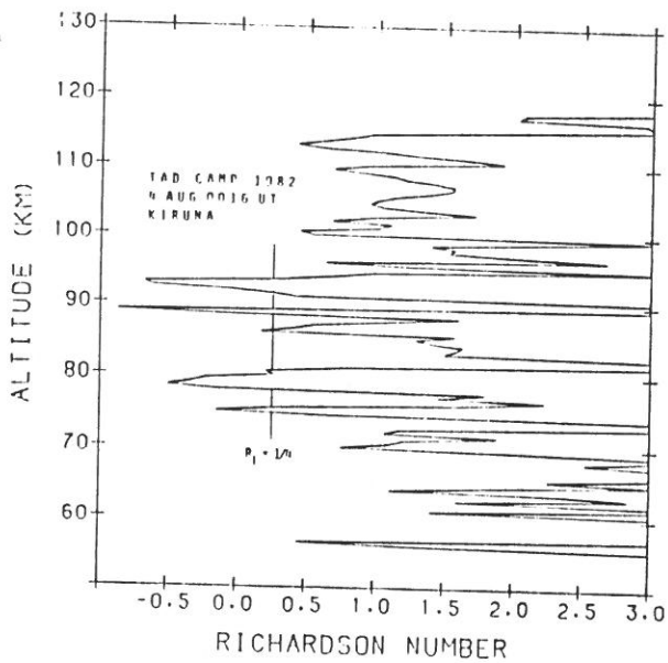
Fig. 2. Richardson numbers inferred from temperatures and horizontal wind velocity measurements during CAMP, in salvo A, on Aug 3/4, 1982 by the piezoelectric accelerometer technique. The regions with Ri < 1/4 indicate dynamically unstable layers.
