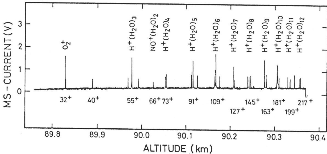
Fig. 5. Positive ion spectrum obtained by the magnetic ion mass spectrometer at 90 km on ascent of rocket flight S 26/1 above Kiruna, on July 30, 1978. (see e.g. Björn et al., 1985).
