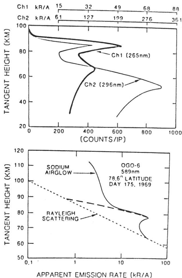
Fig. 1. Limb profiles of PMC taken by the SME ultraviolet spectrometer (upper panel) and the Ogo-6 visible light photometer (lower panel). The ordinate in both figures is the minimum ray height of the line of sight. The lower portions of both data sets are due to scattering from air molecules in the mesosphere. The lower peaks in the UV data are due to O 3 absorption. (Thomas and McKay, 1985)
